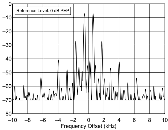
Yaesu FT-100 9D021081 7.250 MHz, Transmit IMD, 100 W F:\SHARED\PROD_REV\TESTS\FT100.2ND\FT100I40.TXT
