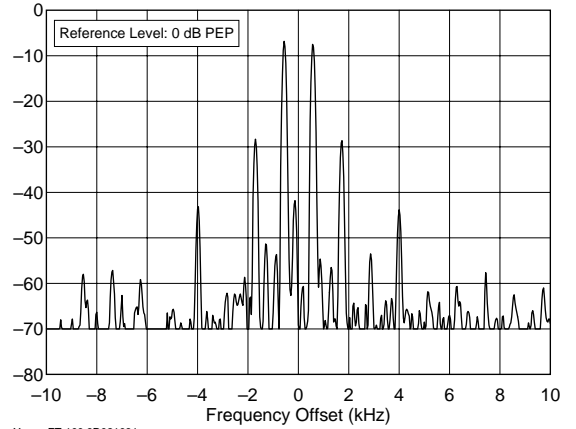
Yaesu FT-100 9D021081 14.250 MHz, Transmit IMD, 100 W F:\SHARED\PROD_REV\TESTS\FT100.2ND\FT100I20.TXT
