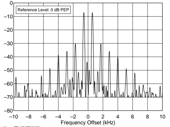
Yaesu FT-100 9D021081 10.120 MHz, Transmit IMD, 100 W F:\SHARED\PROD_REV\TESTS\FT100.2ND\FT100I30.TXT
