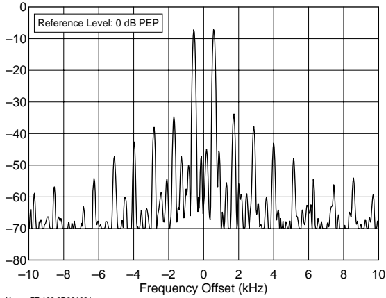
Yaesu FT-100 9D021081 1.350 MHz, Transmit IMD, 100 W F:\SHARED\PROD_REV\TESTS\FT100.2ND\FT100ILO.TXT
