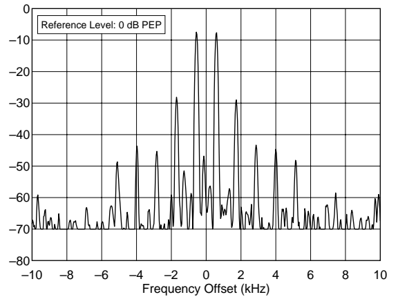
Yaesu FT-100 9D021081 18.120 MHz, Transmit IMD, 100 W F:\SHARED\PROD_REV\TESTS\FT100.2ND\FT100I17.TXT
