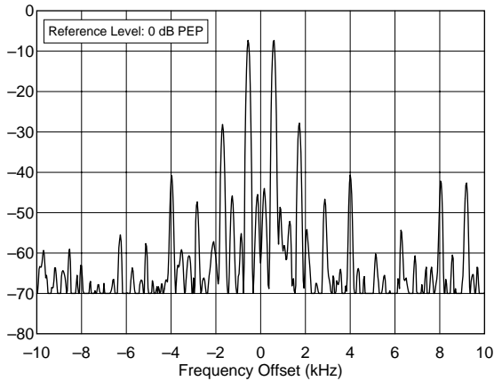
Yaesu FT-100 9D021081 3.950 MHz, Transmit IMD, 100 W F:\SHARED\PROD_REV\TESTS\FT100.2ND\FT100I80.TXT
